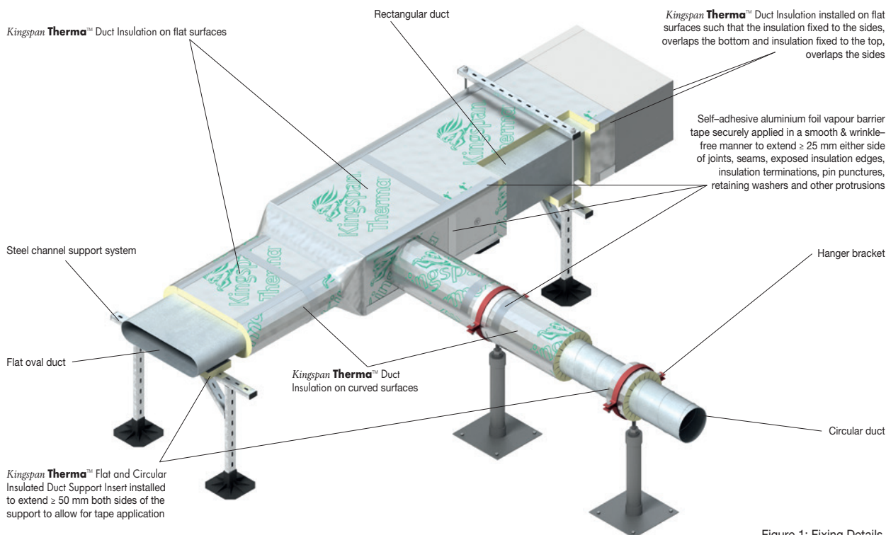
Figure 1: Fixing Details
