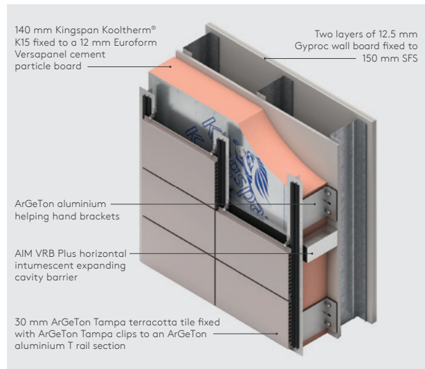
Figure 3: Terracotta Tile Cladding & SFS
